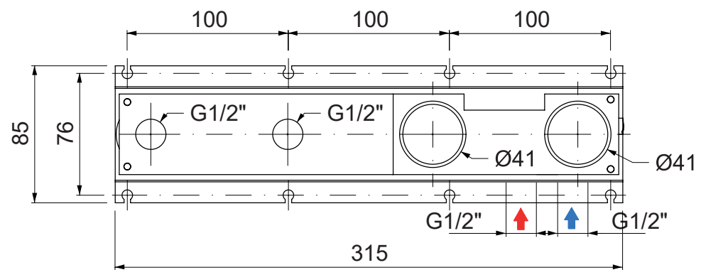
BUILT IN PART - FRONT VIEW
